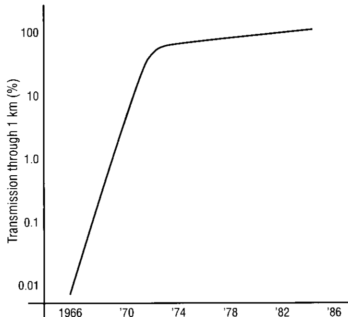
Figure 0.3. Progress in optical fiber transmission. The last two data points represent results near the theoretical limits at 0.85 and 1.55 \mu\text{m} .
