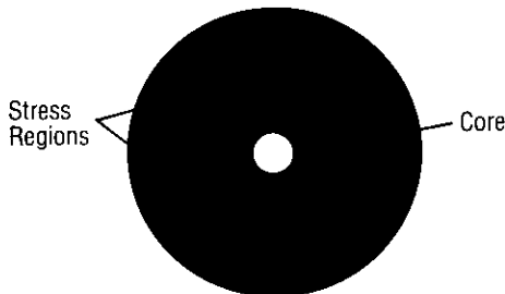
Figure 0.22. Cross section of a polarization-preserving fiber. Stress regions outside the core provide an asymmetry that causes birefringence in the fiber core. Elliptical fibers will also have the same effect.
