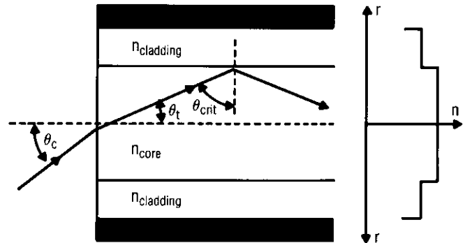
Figure 0.8. Step-index fiber. The refractive index profile is shown at the right. The geometry for derivation of the numerical aperture is given.
