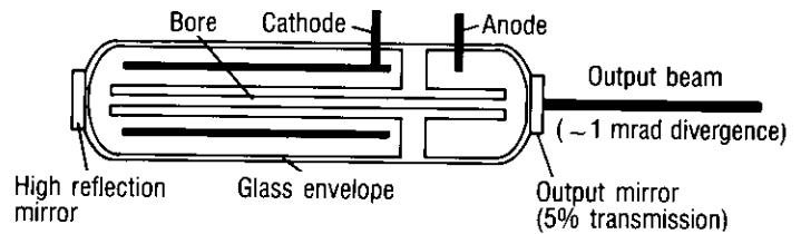
Figure 0.27. Construction of a Helium-Neon laser tube.
