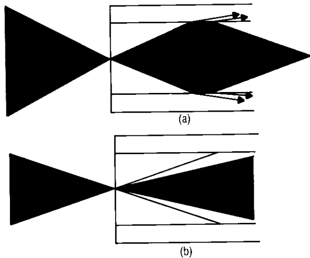
Figure 0.16. Launching conditions in a multimode optical fiber. (a) Overfilled. (b) Underfilled.
