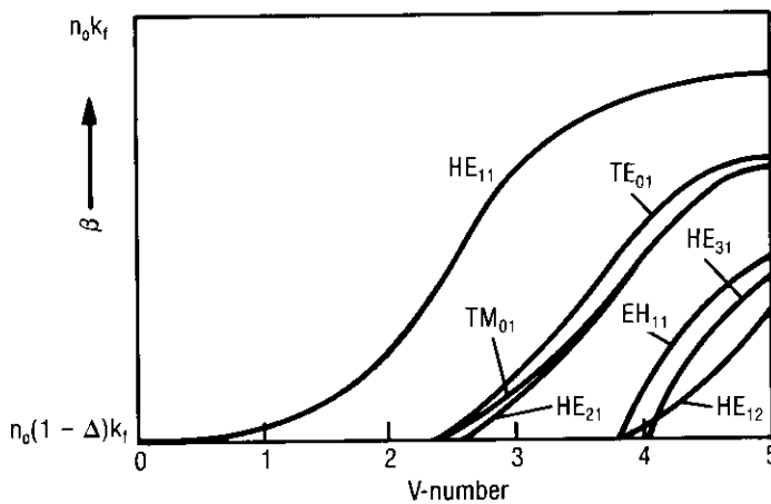
Figure 0.13. Low order modes of an optical fiber. Plot of the propagation constant in a fiber ( \beta ) as a function of V-number of a fiber. Each V-number represents a different fiber configuration or a different wavelength of light in a given fiber configuration. [after D.B. Keck in Fundamentals of Optical Fiber Communication, 2nd Edition, M. K. Barnoski, ed. see references, Copyright © Academic Press, 1981]
